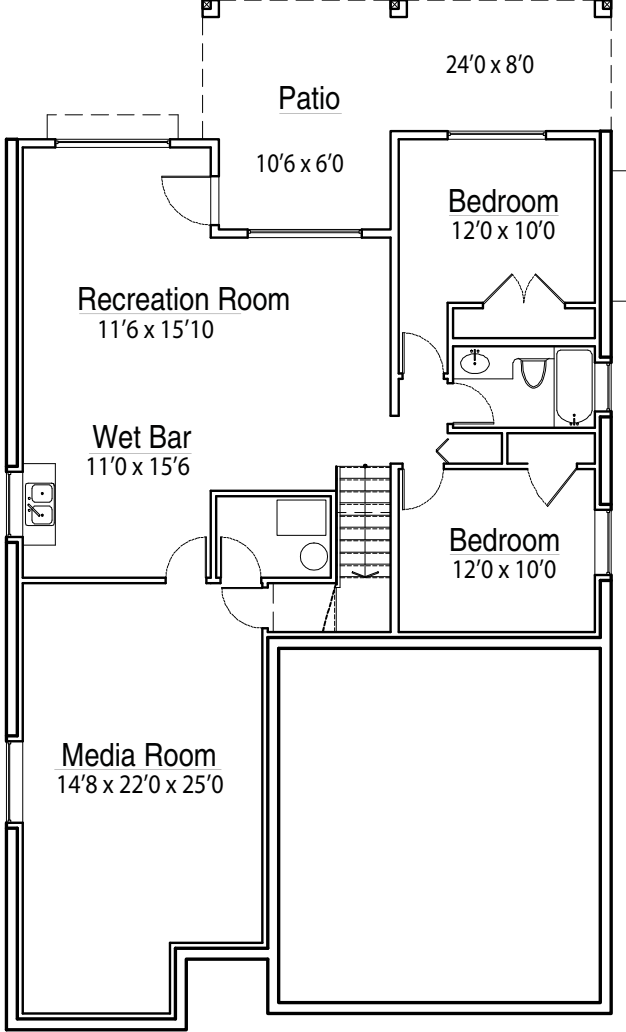
BASEMENT FLOOR: 1,470 sqft. approx.
